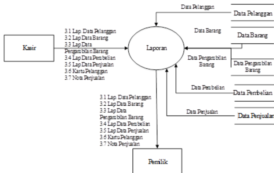
Gambar 5. Diagram DFD Level 0 Proses Laporan
