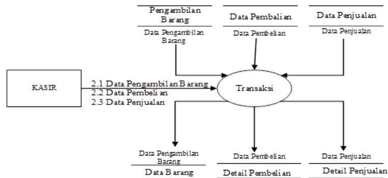
Gambar 4. Diagram DFD Level 0 Proses Transaksi
