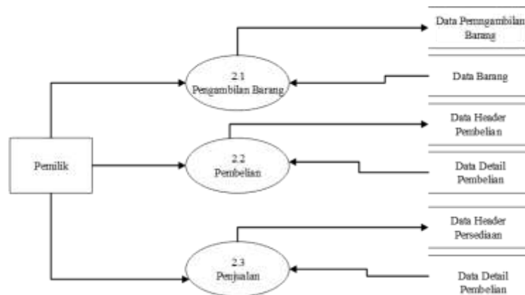
Gambar 7.Diagram DFD Level 1 Proses Transaksi
