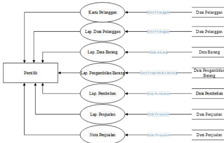
Gambar 8.Diagram DFD Level 1 Proses Laporan
