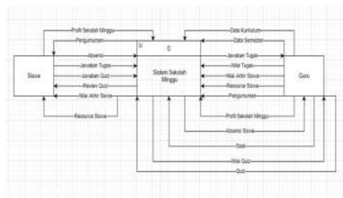
Gambar 4.3 Context Diagram
